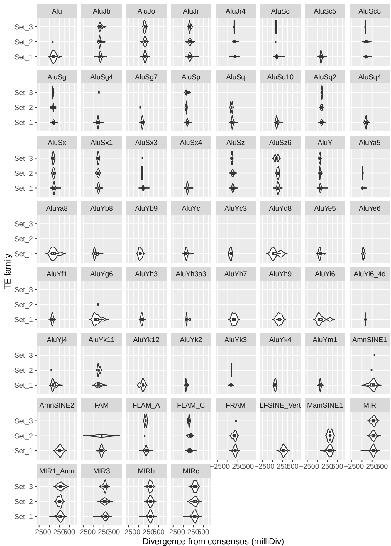
Age distribution of SINE elements overlapping H3K9me3
